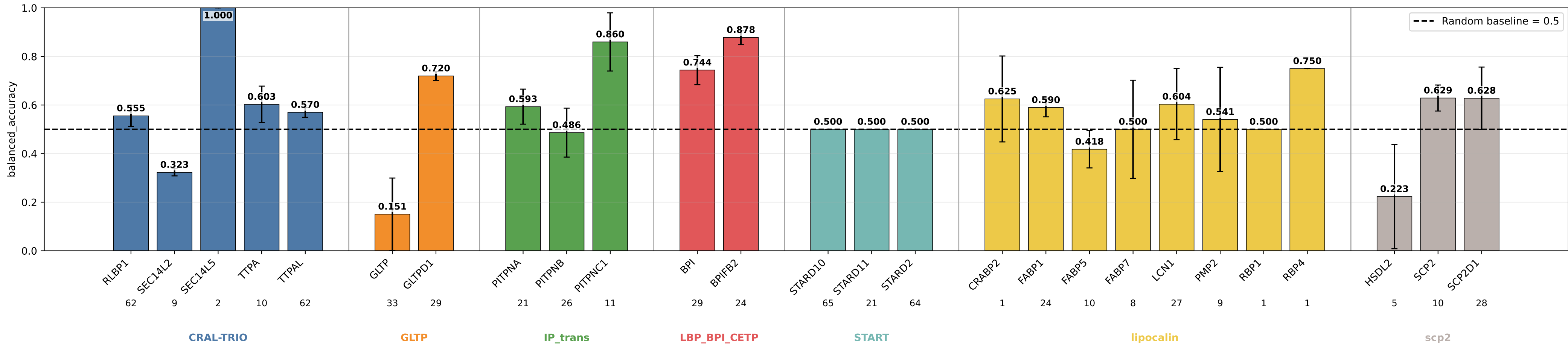
descriptors_path balanced_accuracy by subgroup descriptors_path | class weights | lr=0.0001 | weight_decay=0.01 | final_m=4 | final_dropout=0.1 | hiddim=8 | heads=8 | batch=16 | ep=120 | seeds=0,1
