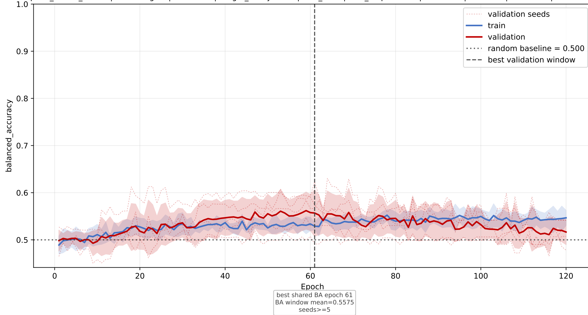
CRAL-TRIO: mean balanced_accuracy learning curve across seeds
