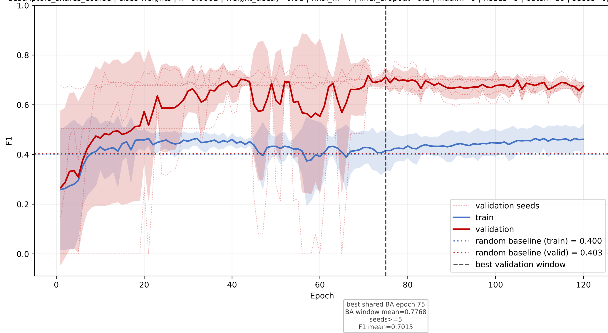
LBP_BPI_CETP: mean F1 learning curve across seeds
