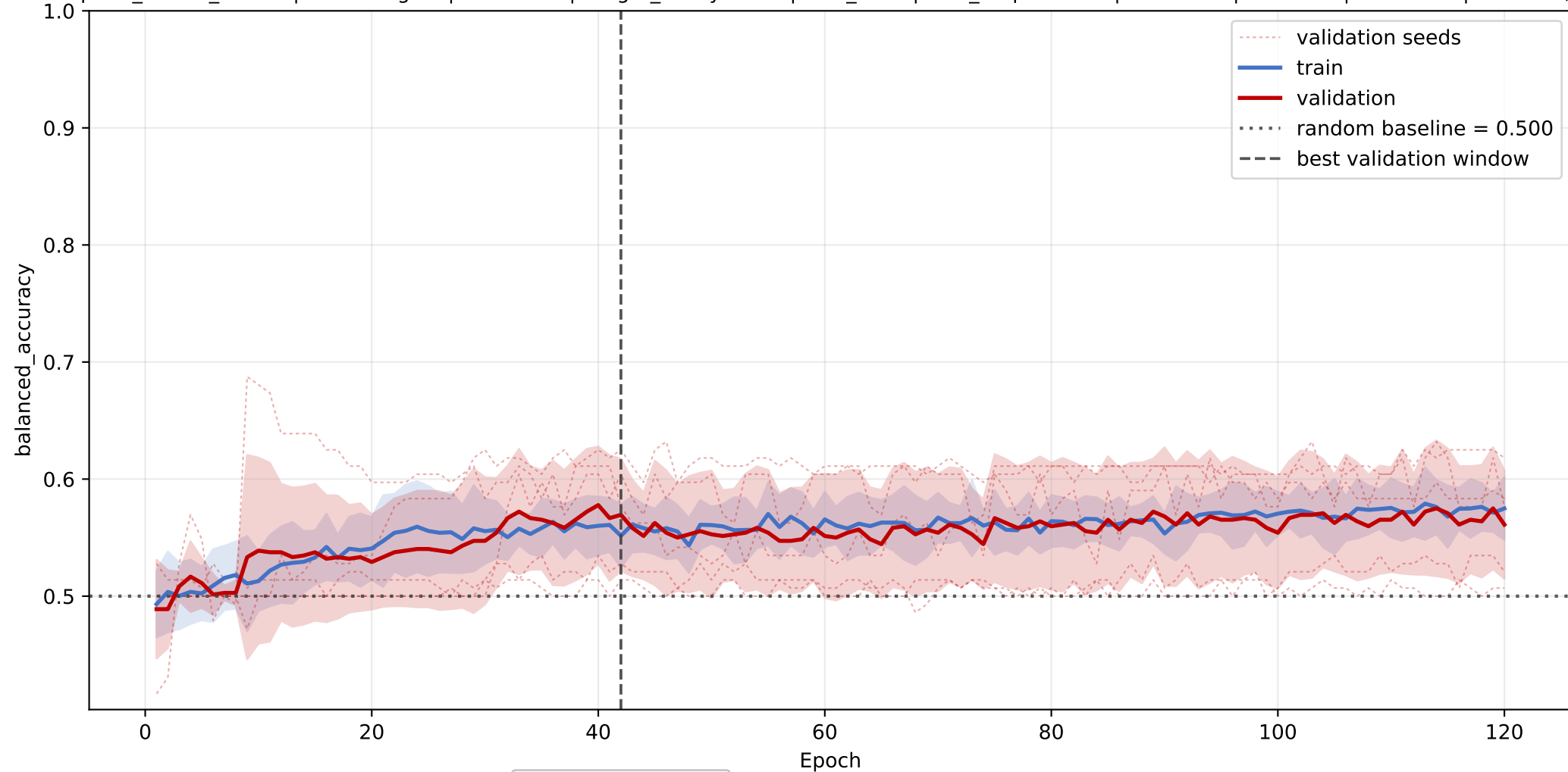
lipocalin: mean balanced_accuracy learning curve across seeds
