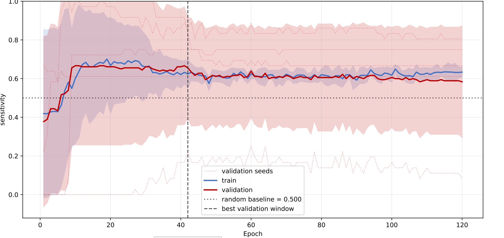
lipocalin: mean sensitivity learning curve across seeds
