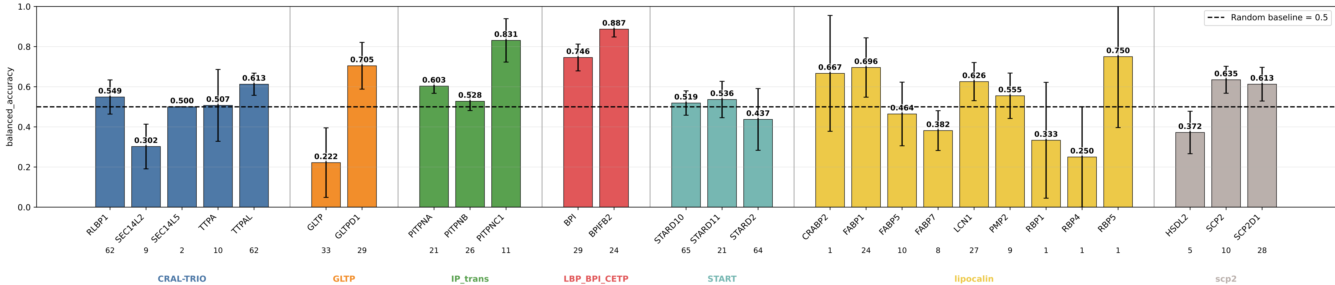
descriptors_shares_coarse balanced_accuracy by subgroup descriptors_shares_coarse | class weights | lr=0.0001 | weight_decay=0.01 | final_m=4 | final_dropout=0.1 | hiddim=8 | heads=8 | batch=16 | ep=120 | seeds=0,1,2,3,4
