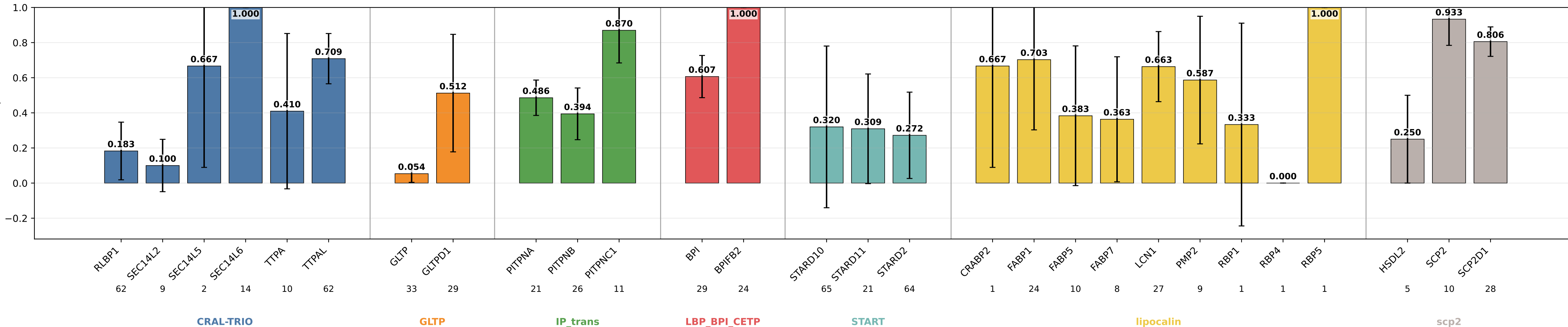
descriptors_shares_coarse sensitivity by subgroup descriptors_shares_coarse | class weights | lr=0.0001 | weight_decay=0.01 | final_m=4 | final_dropout=0.1 | hiddim=8 | heads=8 | batch=16 | ep=120 | seeds=0,1,2,3,4
