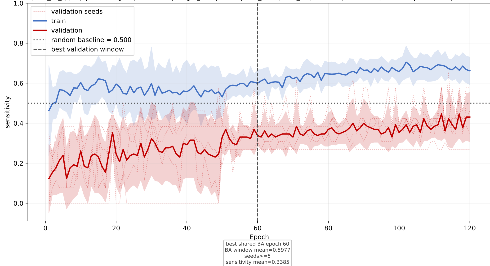
GLTP: mean sensitivity learning curve across seeds
