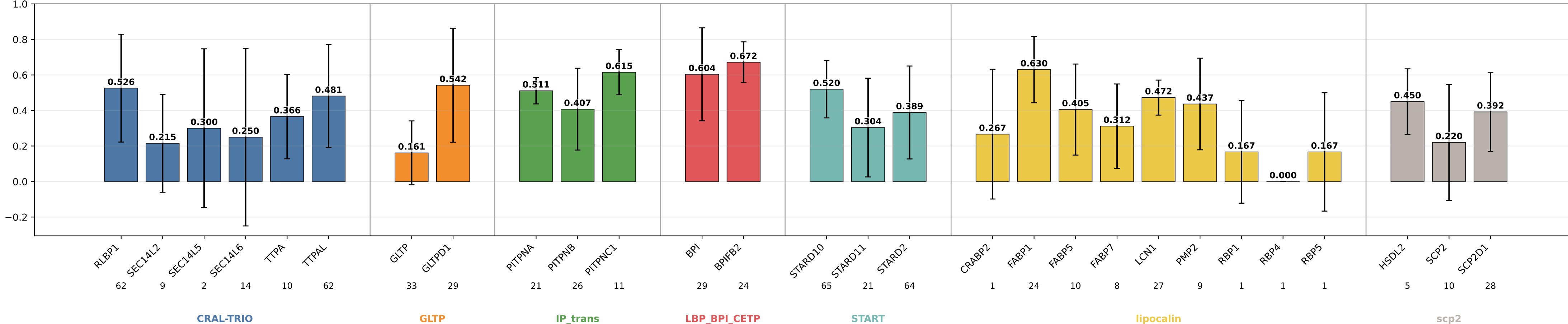
descriptors_v2_lipprop F1 by subgroup descriptors_v2_lipprop | class weights | lr=0.0001 | weight_decay=0.01 | final_m=4 | final_dropout=0.1 | hiddim=8 | heads=8 | batch=16 | ep=120 | seeds=0,1,2,3,4
