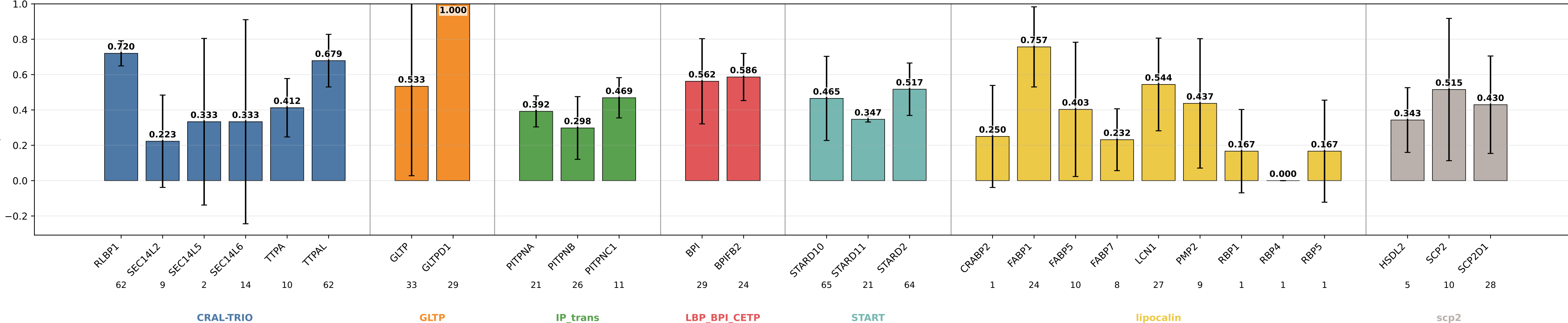
descriptors_v2_lipprop precision by subgroup descriptors_v2_lipprop | class weights | lr=0.0001 | weight_decay=0.01 | final_m=4 | final_dropout=0.1 | hiddim=8 | heads=8 | batch=16 | ep=120 | seeds=0,1,2,3,4
