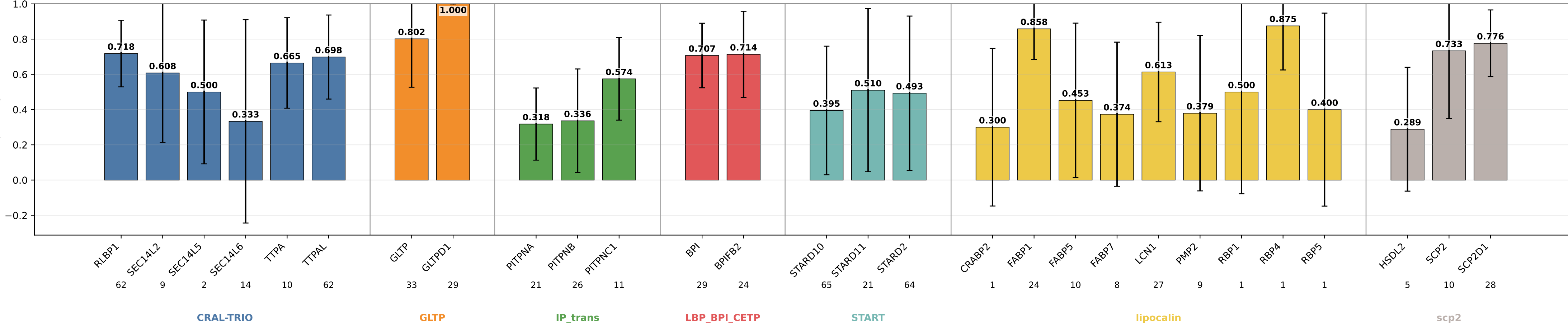
descriptors_v2_lipprop specificity by subgroup descriptors_v2_lipprop | class weights | lr=0.0001 | weight_decay=0.01 | final_m=4 | final_dropout=0.1 | hiddim=8 | heads=8 | batch=16 | ep=120 | seeds=0,1,2,3,4
