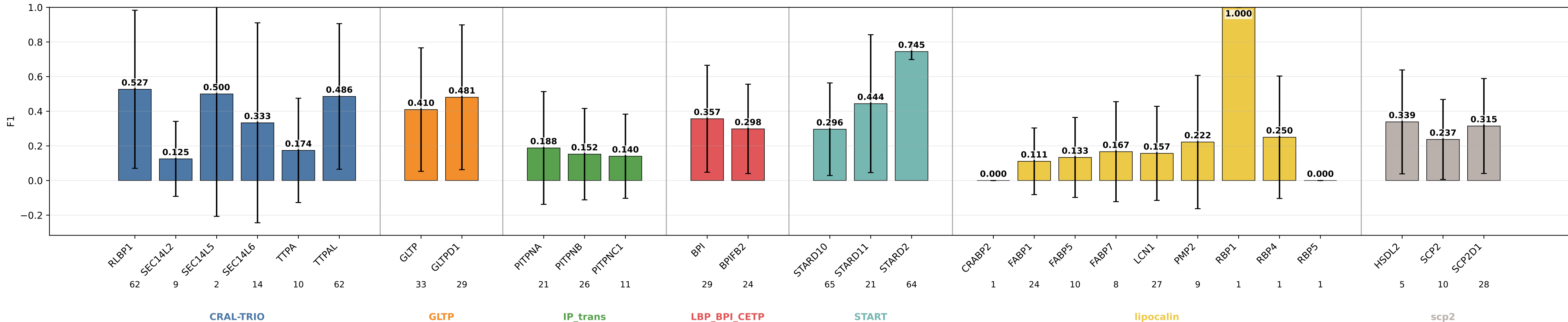
geometric_edge_attention_full F1 by subgroup geometric_edge_attention_full | class weights | lr=0.0001 | weight_decay=0.01 | final_m=4 | final_dropout=0.1 | hiddim=8 | heads=8 | batch=16 | ep=120 | seeds=0,1,2
