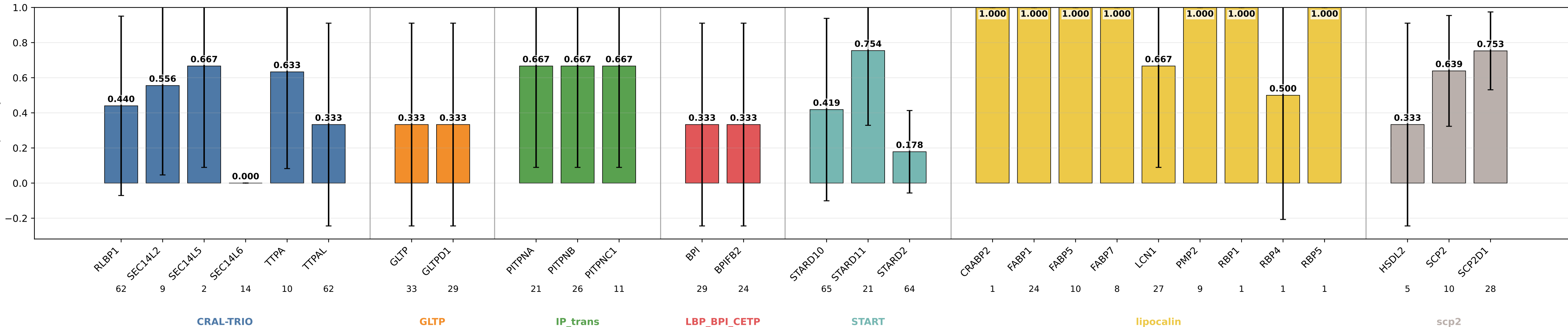
geometric_edge_attention_full specificity by subgroup geometric_edge_attention_full | class weights | lr=0.0001 | weight_decay=0.01 | final_m=4 | final_dropout=0.1 | hiddim=8 | heads=8 | batch=16 | ep=120 | seeds=0,1,2
