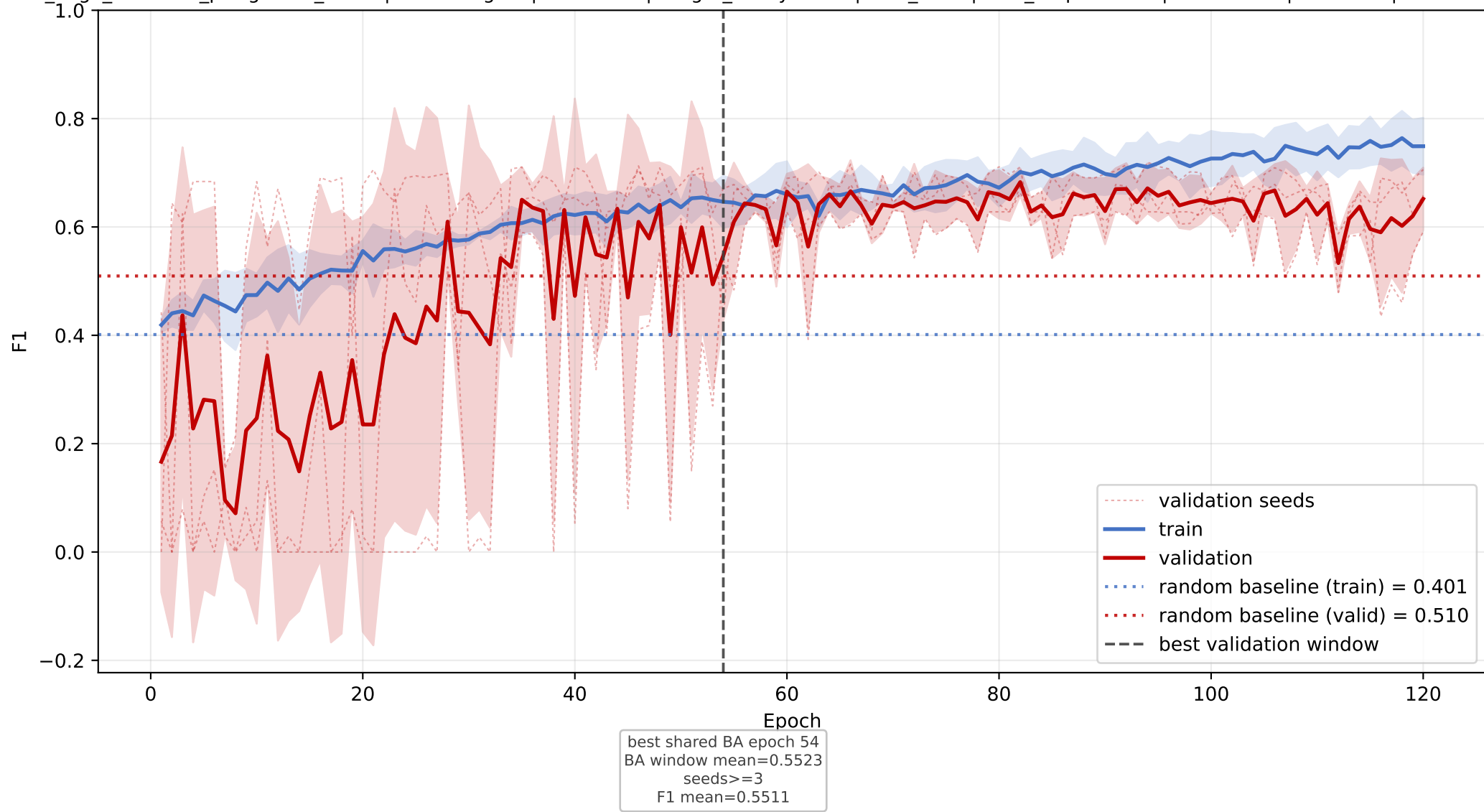
CRAL-TRIO: mean F1 learning curve across seeds
