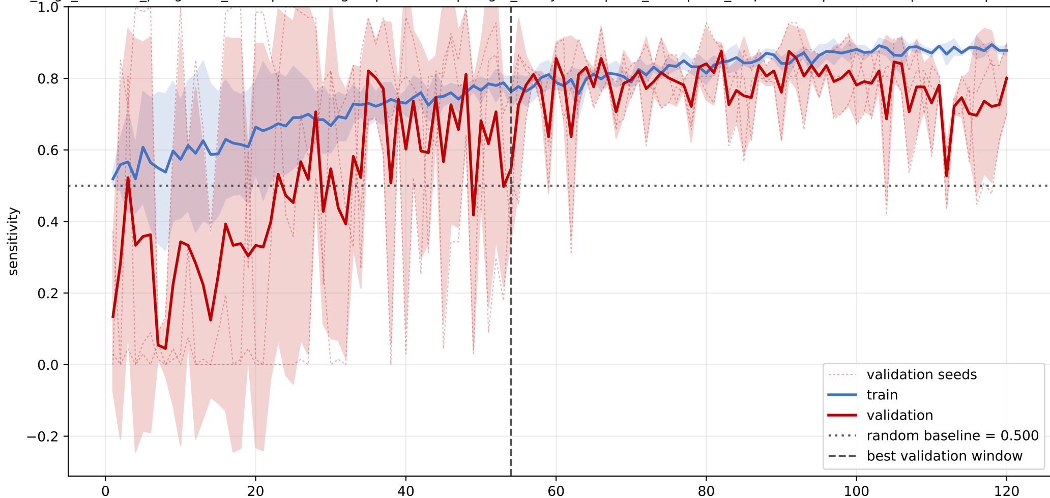
CRAL-TRIO: mean sensitivity learning curve across seeds
