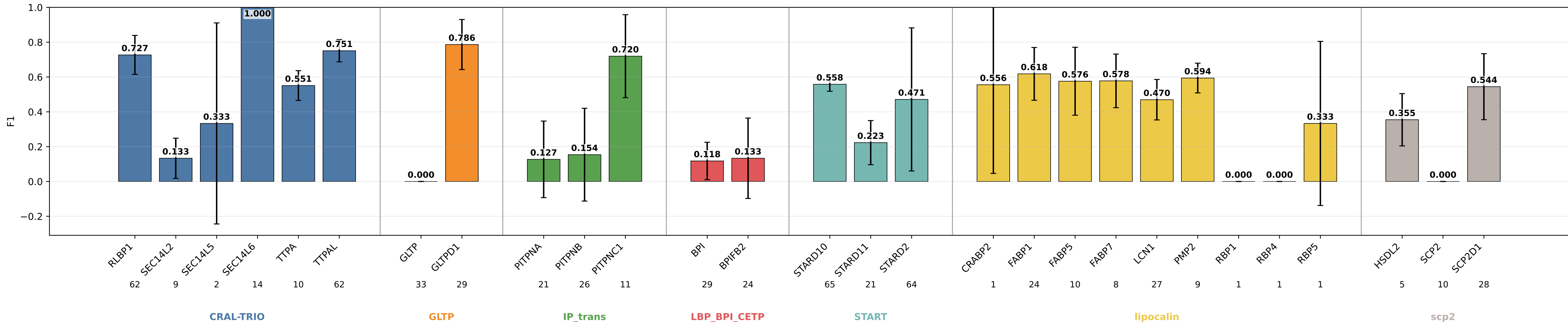
geometric_edge_attention_protgeom8_hid16 F1 by subgroup geometric_edge_attention_protgeom8_hid16 | class weights | lr=0.0001 | weight_decay=0.01 | final_m=4 | final_dropout=0.1 | hiddim=16 | heads=8 | batch=16 | ep=120 | seeds=0,1,2
