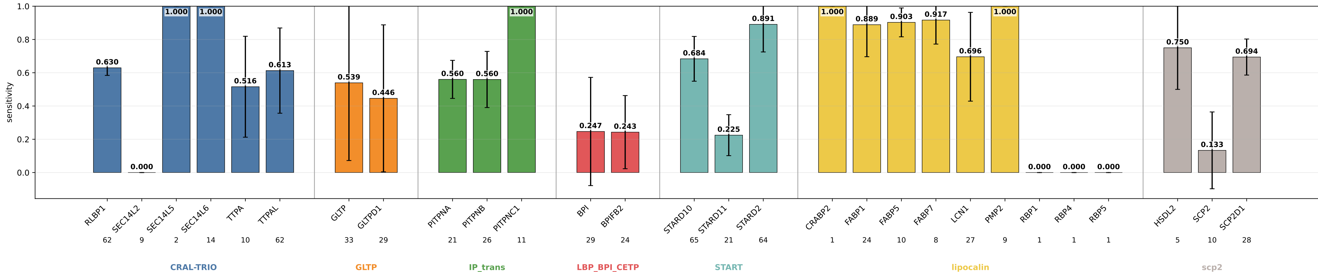
geometric_edge_attention_protgeom8_hid32 sensitivity by subgroup geometric_edge_attention_protgeom8_hid32 | class weights | lr=0.0001 | weight_decay=0.01 | final_m=4 | final_dropout=0.1 | hiddim=32 | heads=8 | batch=16 | ep=120 | seeds=0,1,2
