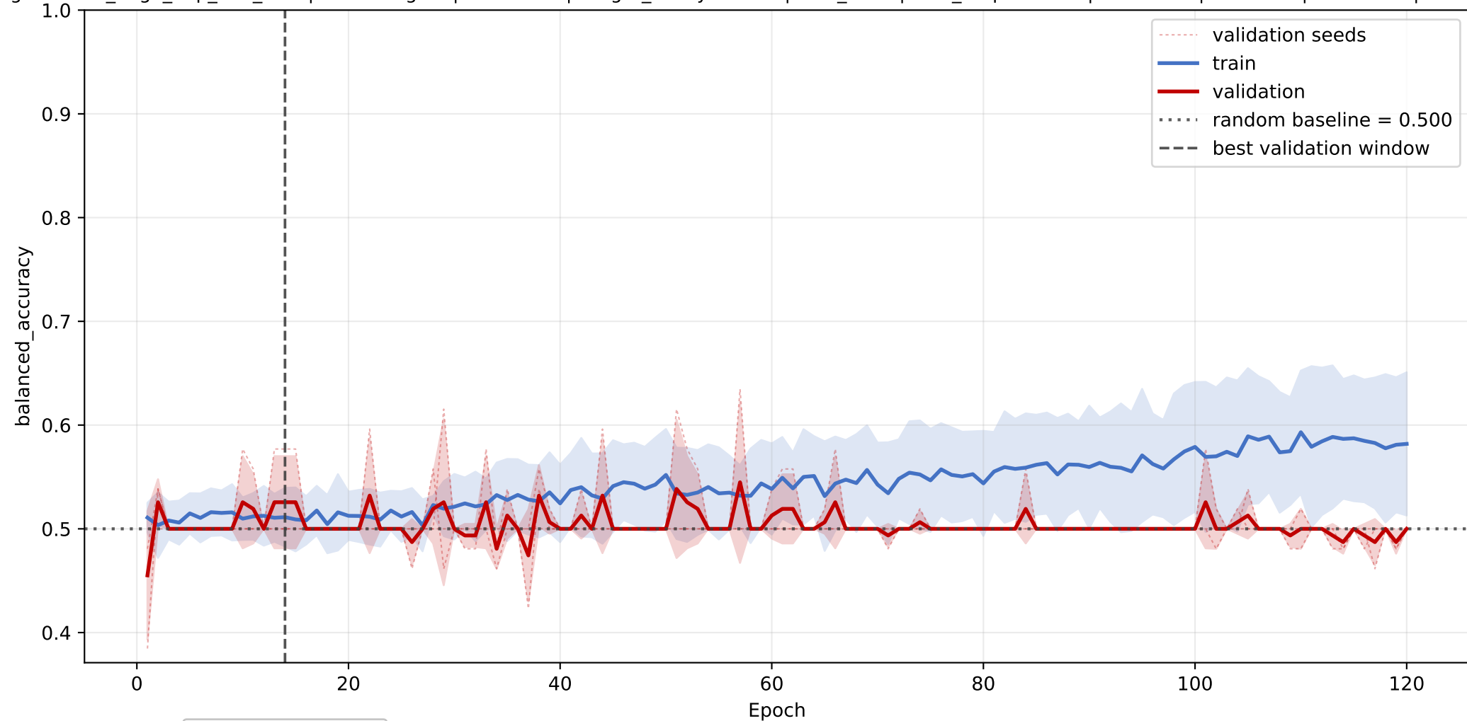
GLTP: mean balanced_accuracy learning curve across seeds
