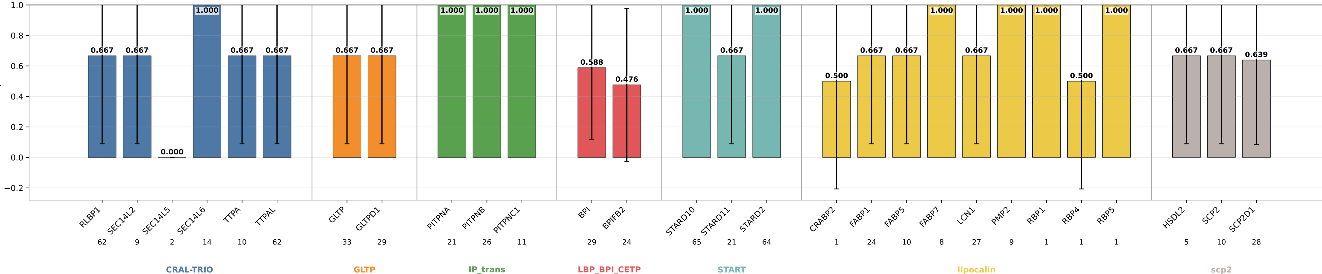
geometric_edge_mlp_full sensitivity by subgroup geometric_edge_mlp_full | class weights | lr=0.0001 | weight_decay=0.01 | final_m=4 | final_dropout=0.1 | hiddim=8 | heads=8 | batch=16 | ep=120 | seeds=0,1,2
