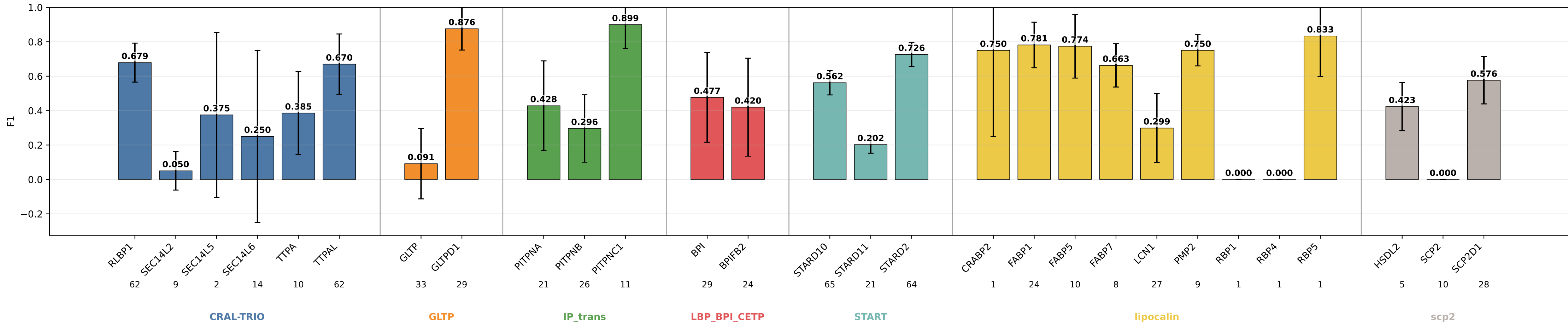
geometric_edge_mlp_protgeom8 F1 by subgroup geometric_edge_mlp_protgeom8 | class weights | lr=0.0001 | weight_decay=0.01 | final_m=4 | final_dropout=0.1 | hiddim=8 | heads=8 | batch=16 | ep=120 | seeds=0,1,2,3,4
