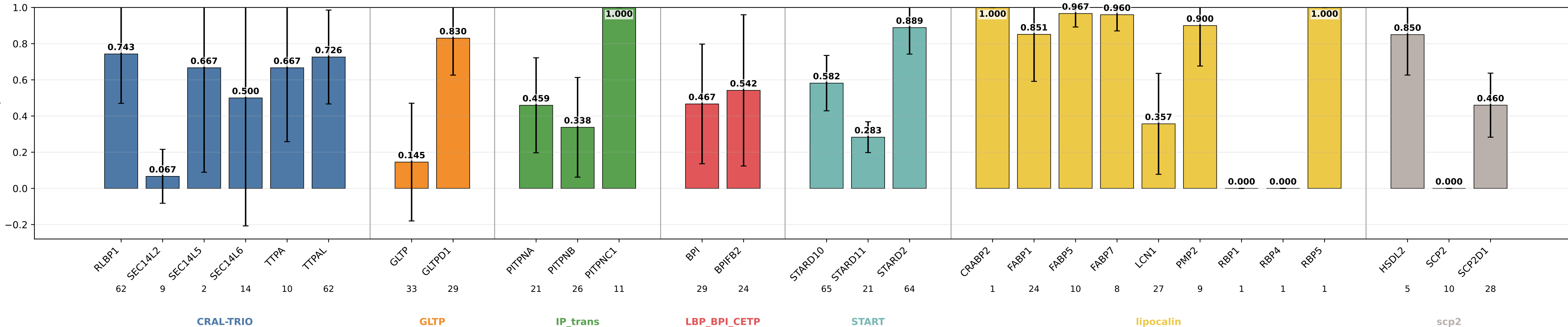
geometric_edge_mlp_protgeom8 sensitivity by subgroup geometric_edge_mlp_protgeom8 | class weights | lr=0.0001 | weight_decay=0.01 | final_m=4 | final_dropout=0.1 | hiddim=8 | heads=8 | batch=16 | ep=120 | seeds=0,1,2,3,4
