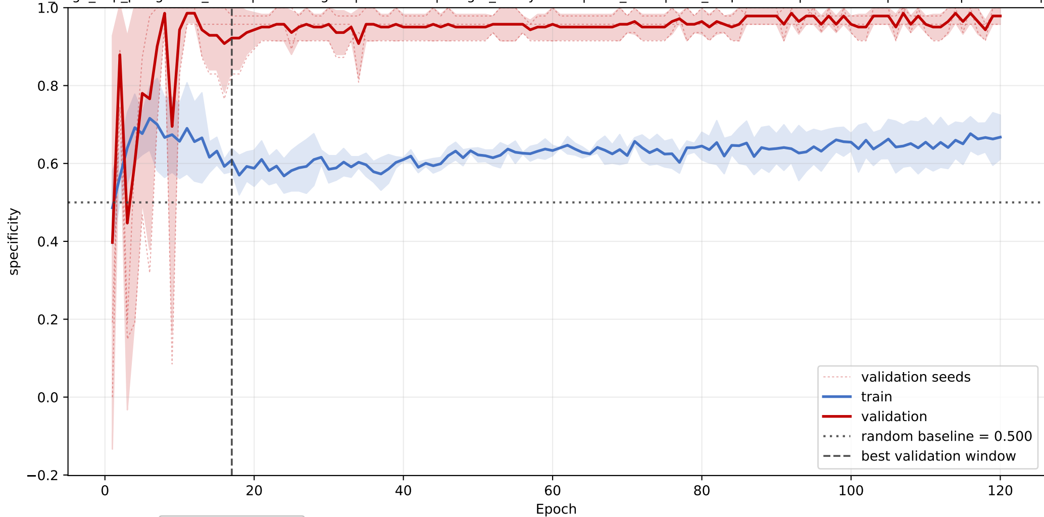
LBP_BPI_CETP: mean specificity learning curve across seeds
