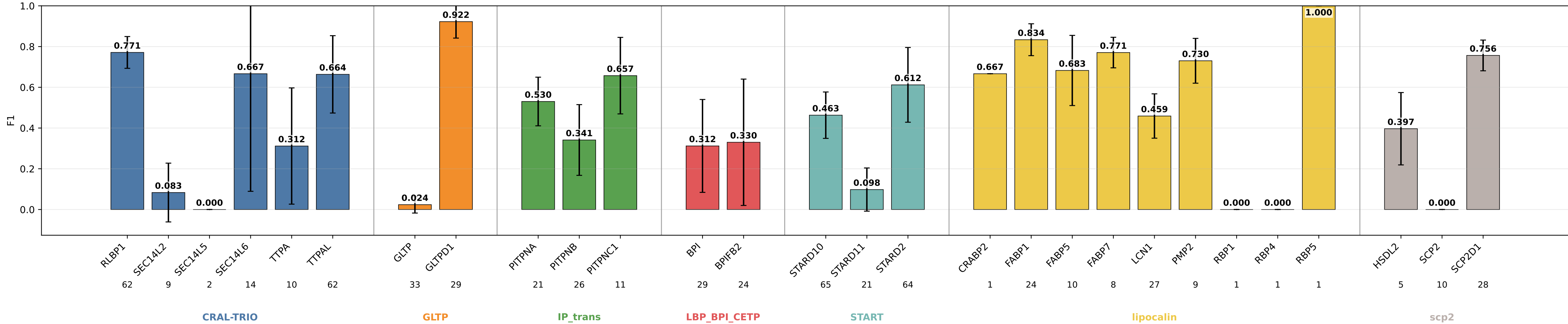
geometric_edge_mlp_protgeom8_hid16 F1 by subgroup geometric_edge_mlp_protgeom8_hid16 | class weights | lr=0.0001 | weight_decay=0.01 | final_m=4 | final_dropout=0.1 | hiddim=16 | heads=8 | batch=16 | ep=120 | seeds=0,1,2
