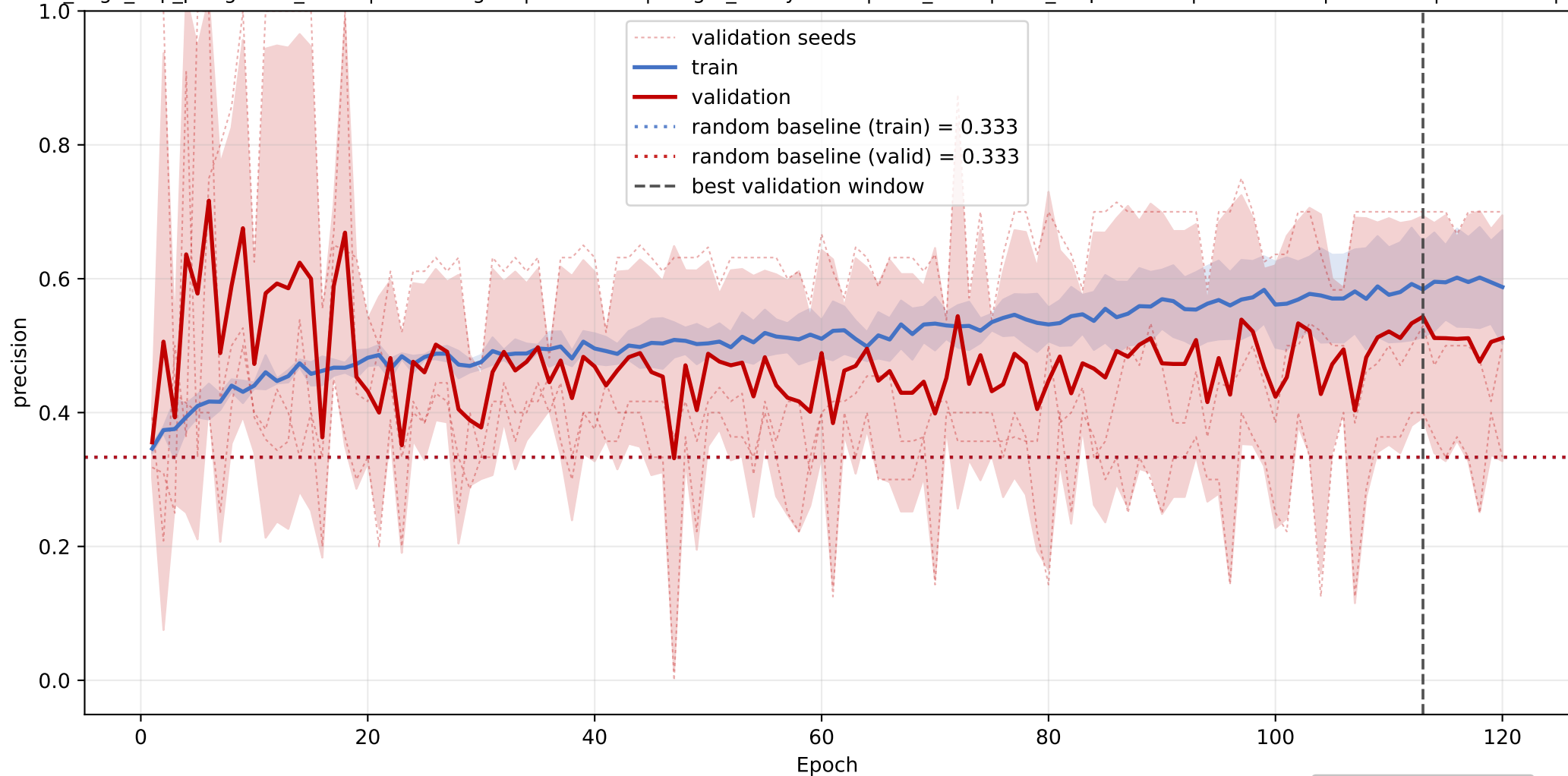
scp2: mean precision learning curve across seeds
