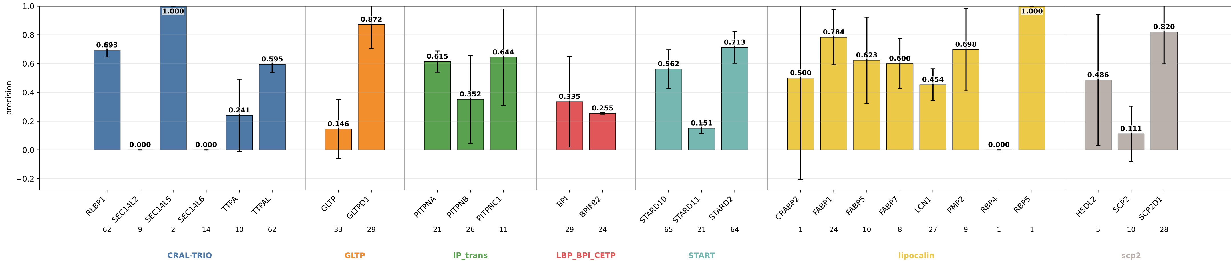
geometric_edge_mlp_protgeom8_hid32 precision by subgroup geometric_edge_mlp_protgeom8_hid32 | class weights | lr=0.0001 | weight_decay=0.01 | final_m=4 | final_dropout=0.1 | hiddim=32 | heads=8 | batch=16 | ep=120 | seeds=0,1,2
