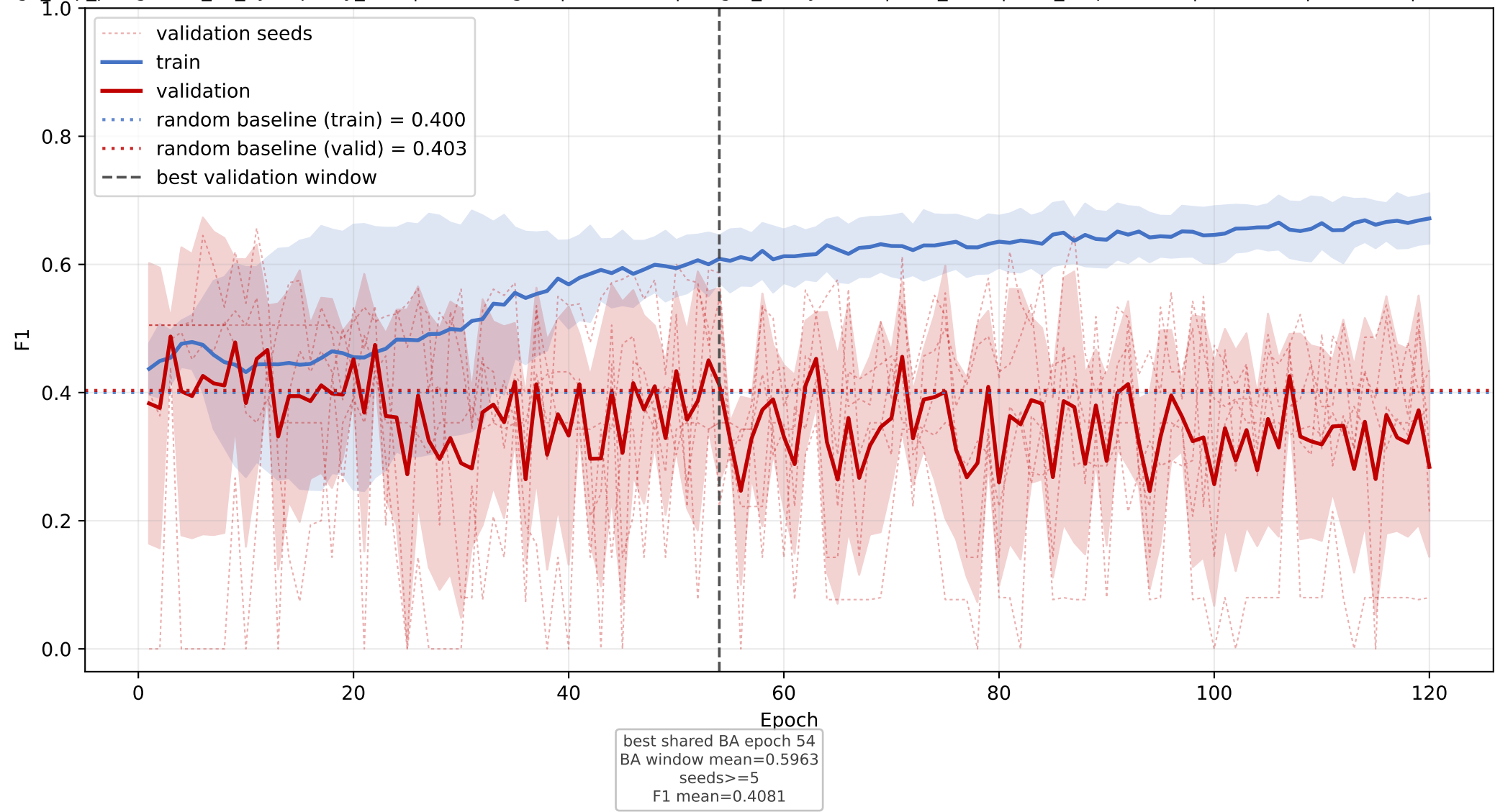
IP_trans: mean F1 learning curve across seeds
