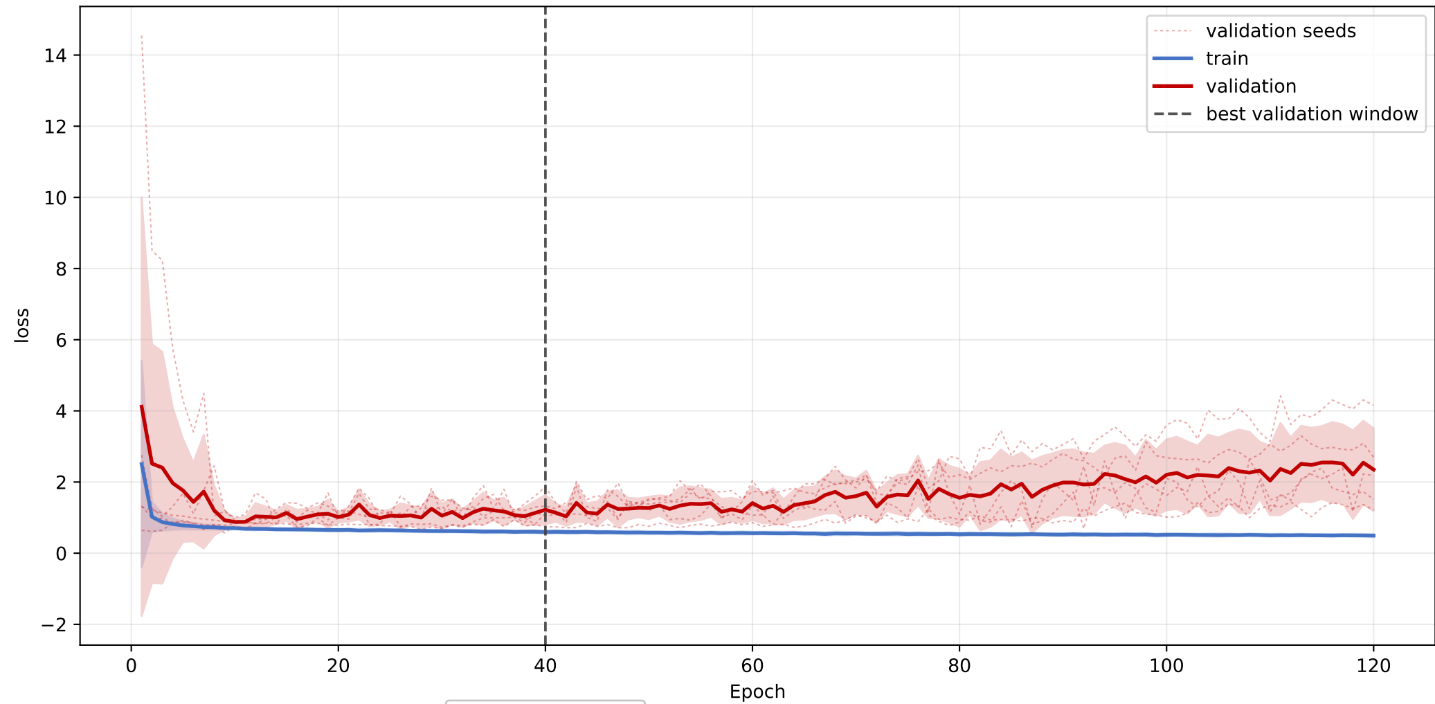
LBP_BPI_CETP: mean loss learning curve across seeds
