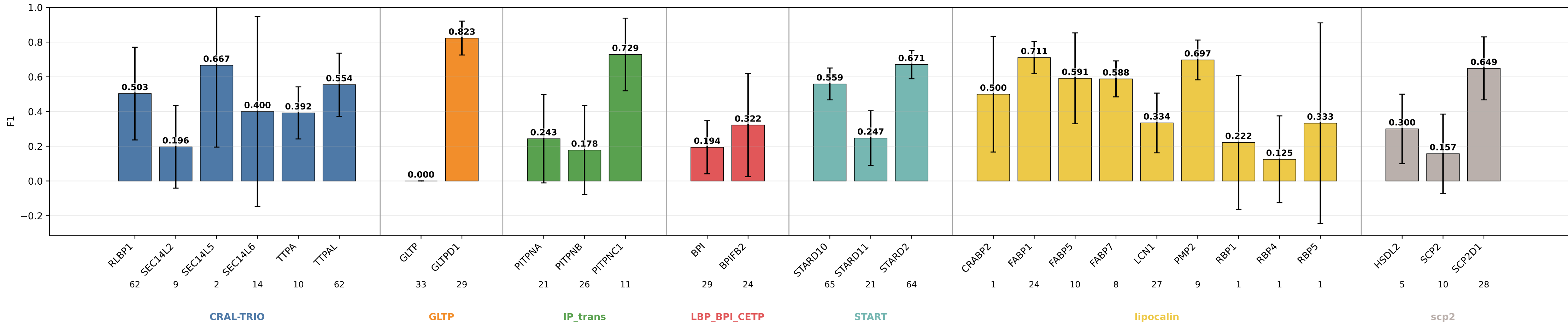
geometric_edge_mlp_protgeom8_no_hydropathy_core F1 by subgroup geometric_edge_mlp_protgeom8_no_hydropathy_core | class weights | lr=0.0001 | weight_decay=0.01 | final_m=4 | final_dropout=0.1 | hiddim=8 | heads=8 | batch=16 | ep=120 | seeds=0,1,2,3,4
