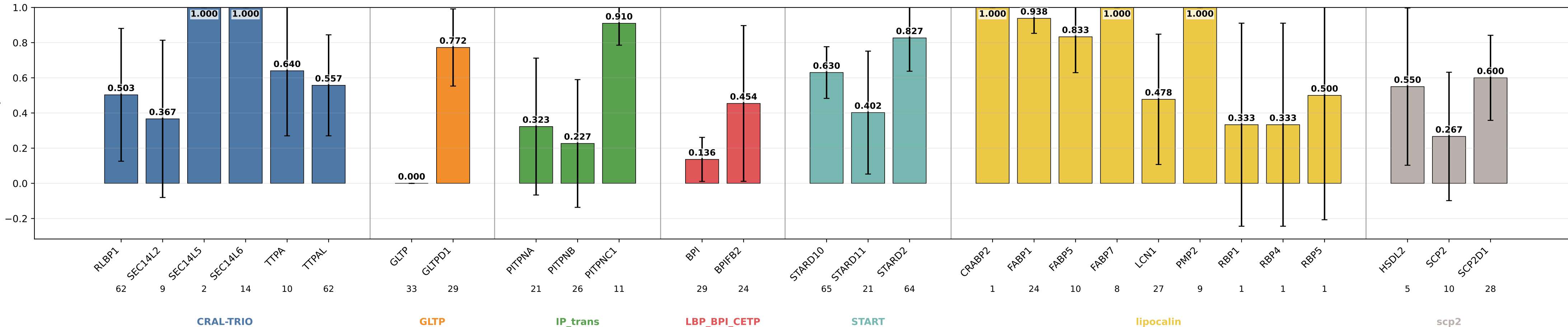
geometric_edge_mlp_protgeom8_no_hydropathy_core sensitivity by subgroup geometric_edge_mlp_protgeom8_no_hydropathy_core | class weights | lr=0.0001 | weight_decay=0.01 | final_m=4 | final_dropout=0.1 | hiddim=8 | heads=8 | batch=16 | ep=120 | seeds=0,1,2,3,4
