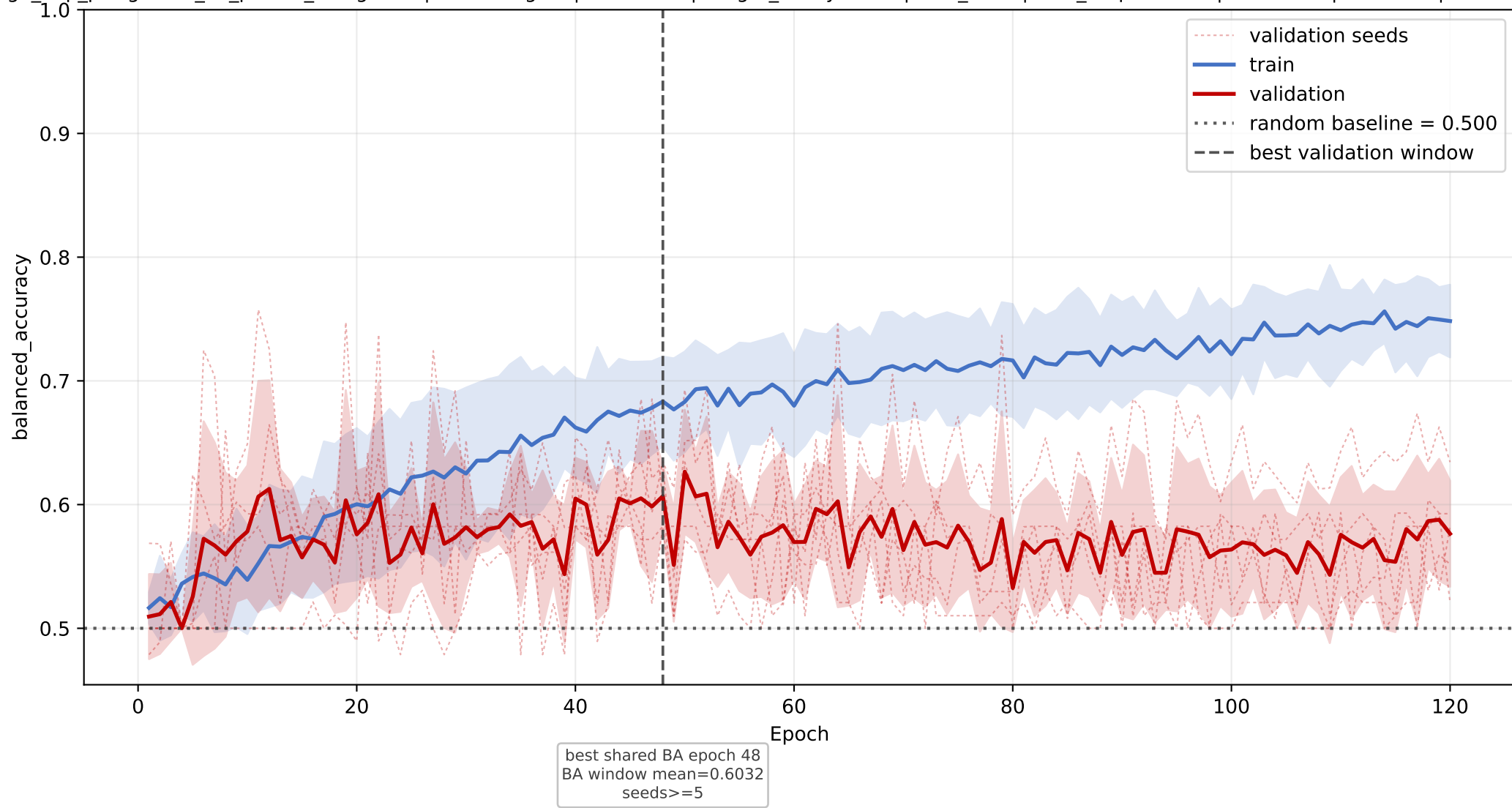
IP_trans: mean balanced_accuracy learning curve across seeds
