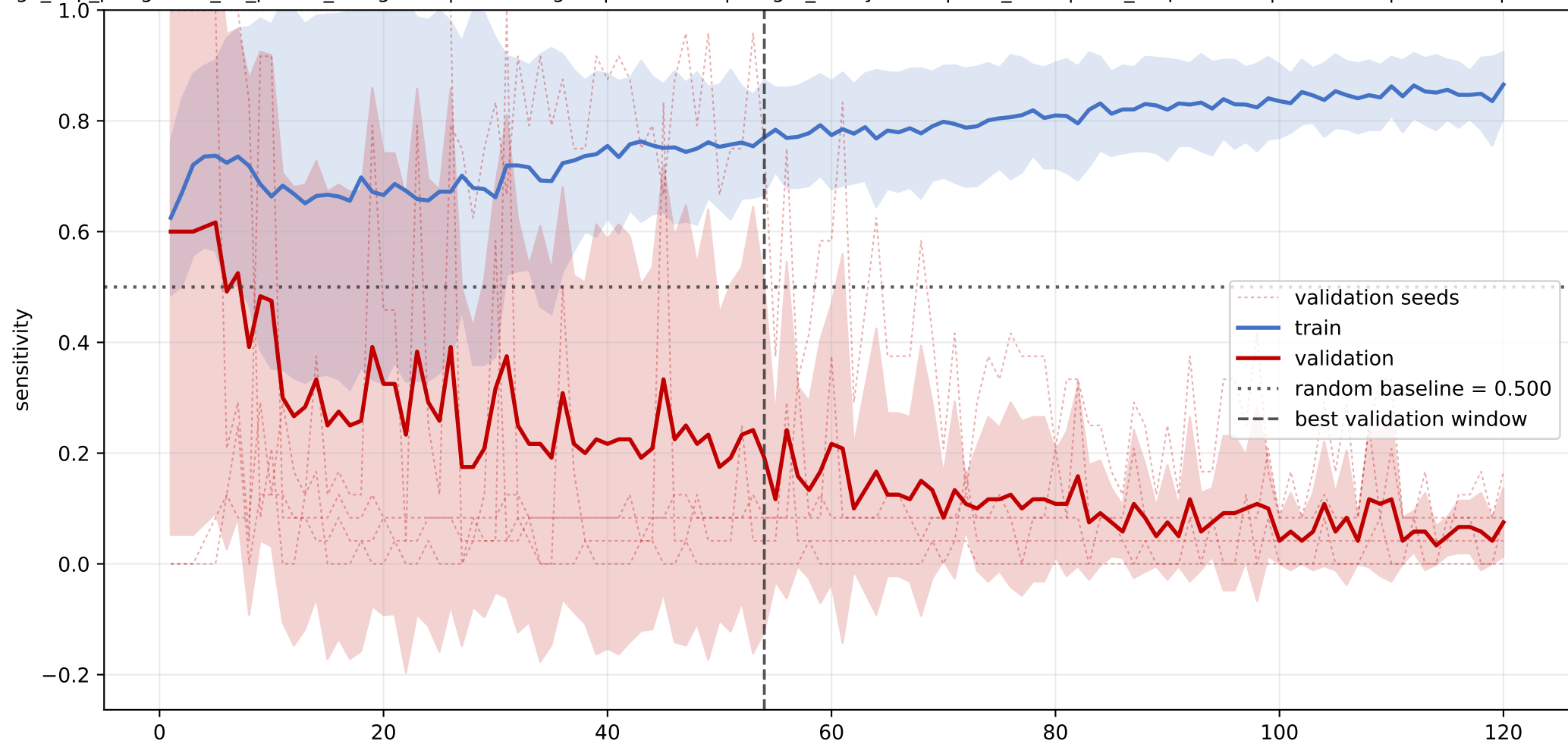
LBP_BPI_CETP: mean sensitivity learning curve across seeds
