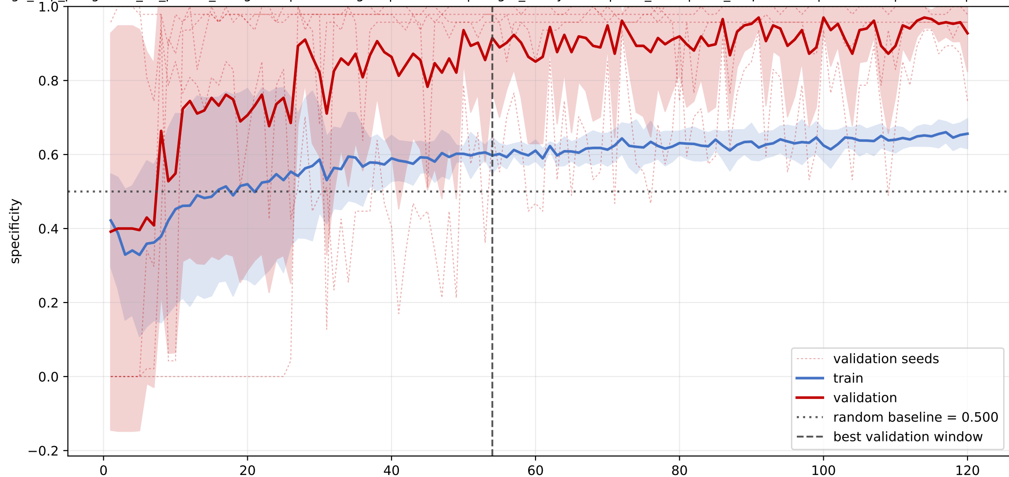
LBP_BPI_CETP: mean specificity learning curve across seeds
