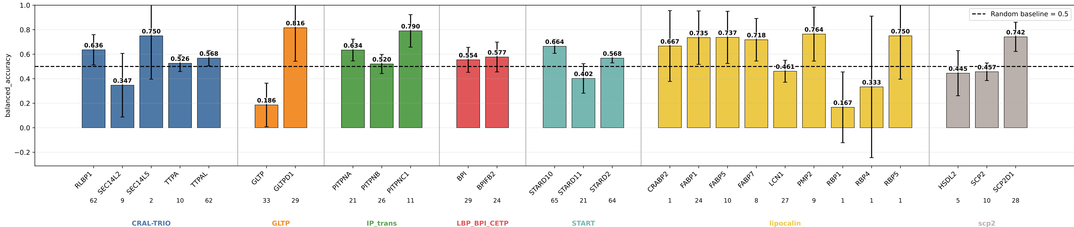
geometric_edge_mlp_protgeom8_no_pocket_elongation balanced_accuracy by subgroup geometric_edge_mlp_protgeom8_no_pocket_elongation | class weights | lr=0.0001 | weight_decay=0.01 | final_m=4 | final_dropout=0.1 | hiddim=8 | heads=8 | batch=16 | ep=120 | seeds=0,1,2,3,4
