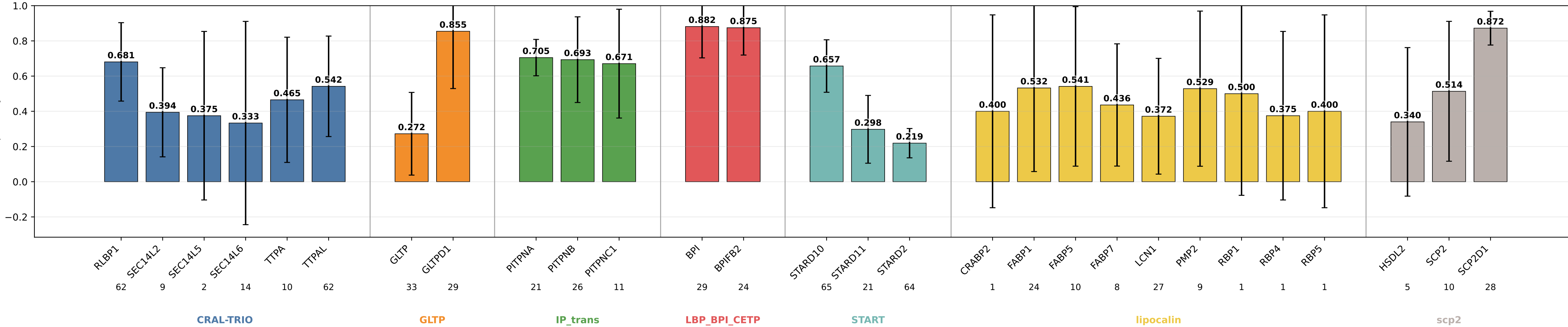
geometric_edge_mlp_protgeom8_no_pocket_elongation specificity by subgroup geometric_edge_mlp_protgeom8_no_pocket_elongation | class weights | lr=0.0001 | weight_decay=0.01 | final_m=4 | final_dropout=0.1 | hiddim=8 | heads=8 | batch=16 | ep=120 | seeds=0,1,2,3,4
