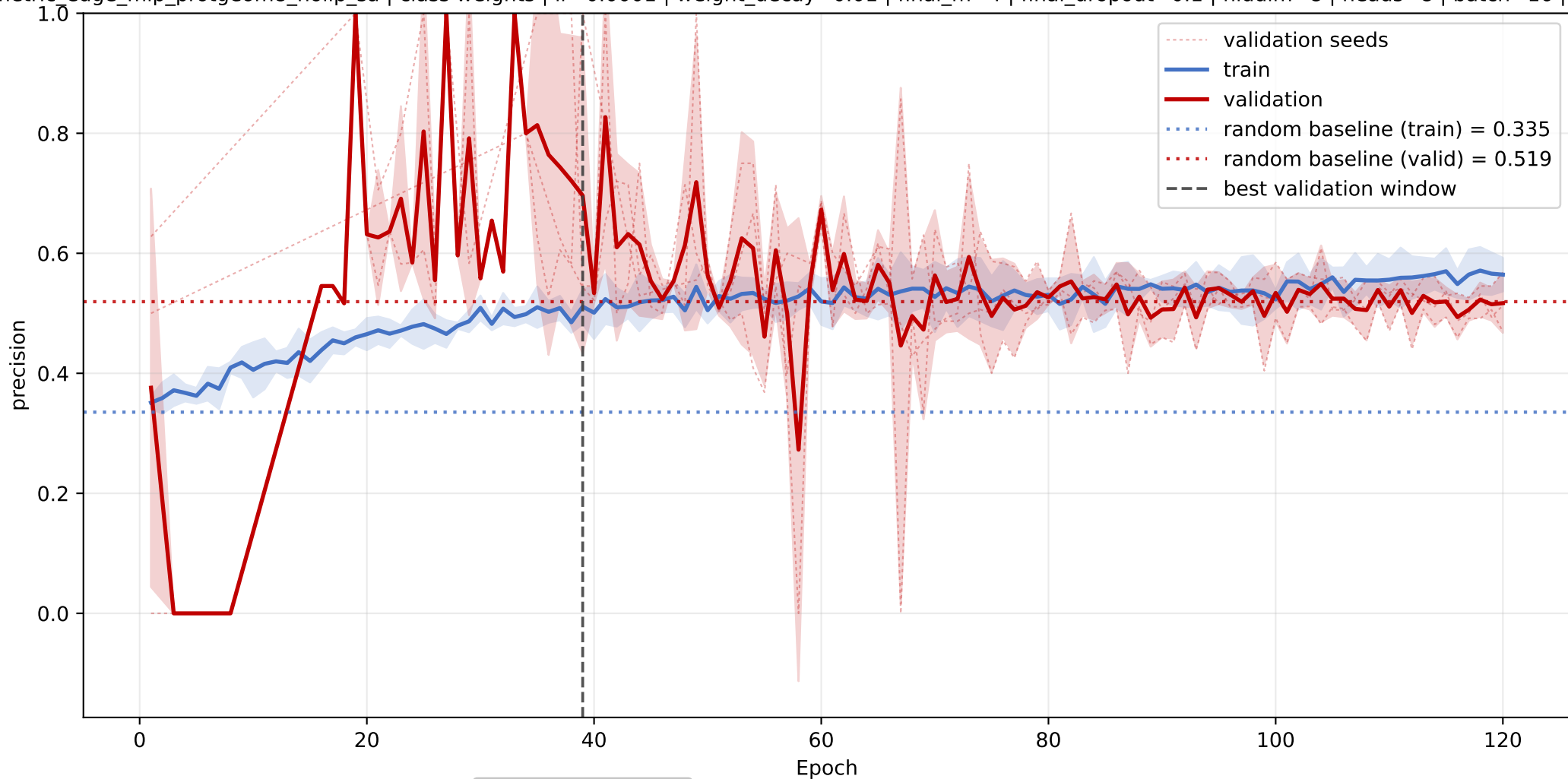
CRAL-TRIO: mean precision learning curve across seeds
