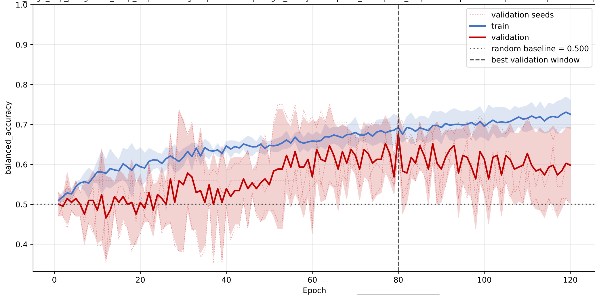
scp2: mean balanced_accuracy learning curve across seeds
