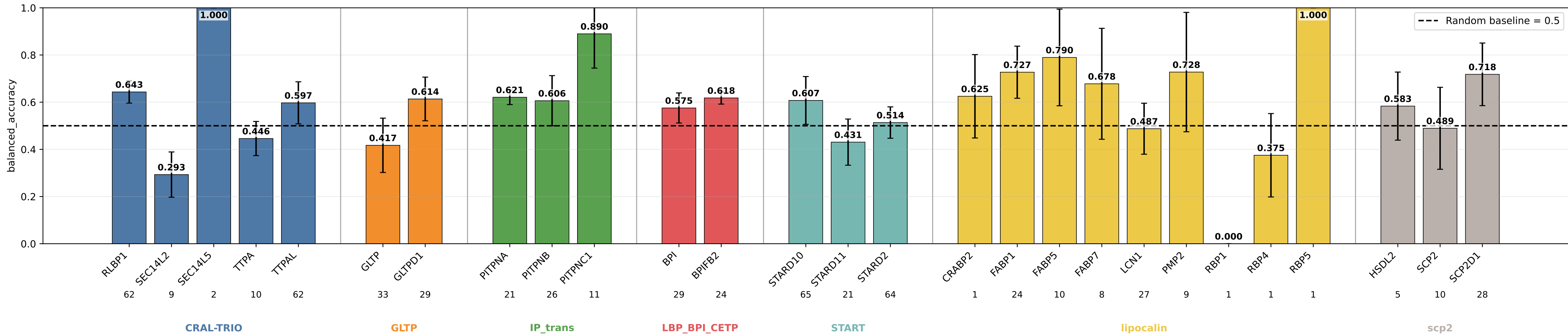
geometric_edge_mlp_protgeom8_nolip_sa balanced_accuracy by subgroup geometric_edge_mlp_protgeom8_nolip_sa | class weights | lr=0.0001 | weight_decay=0.01 | final_m=4 | final_dropout=0.1 | hiddim=8 | heads=8 | batch=16 | ep=120 | seeds=0,1,2
