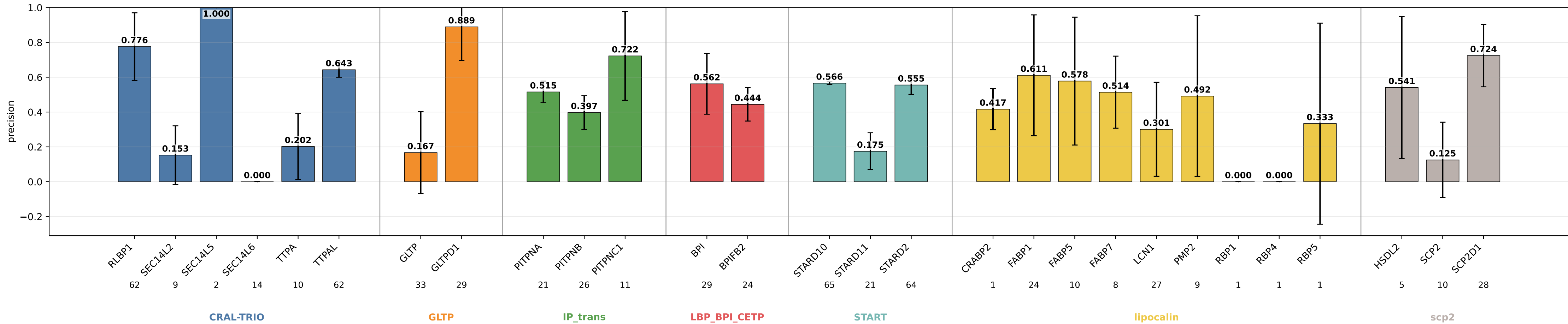
geometric_edge_mlp_protgeom8_nolip_sa precision by subgroup geometric_edge_mlp_protgeom8_nolip_sa | class weights | lr=0.0001 | weight_decay=0.01 | final_m=4 | final_dropout=0.1 | hiddim=8 | heads=8 | batch=16 | ep=120 | seeds=0,1,2
