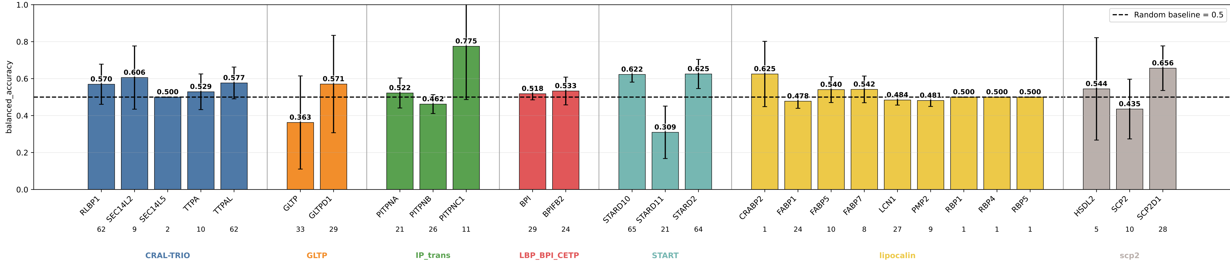
geometric_edge_mlp_protgeom8_noprot_sa balanced_accuracy by subgroup geometric_edge_mlp_protgeom8_noprot_sa | class weights | lr=0.0001 | weight_decay=0.01 | final_m=4 | final_dropout=0.1 | hiddim=8 | heads=8 | batch=16 | ep=120 | seeds=0,1,2
