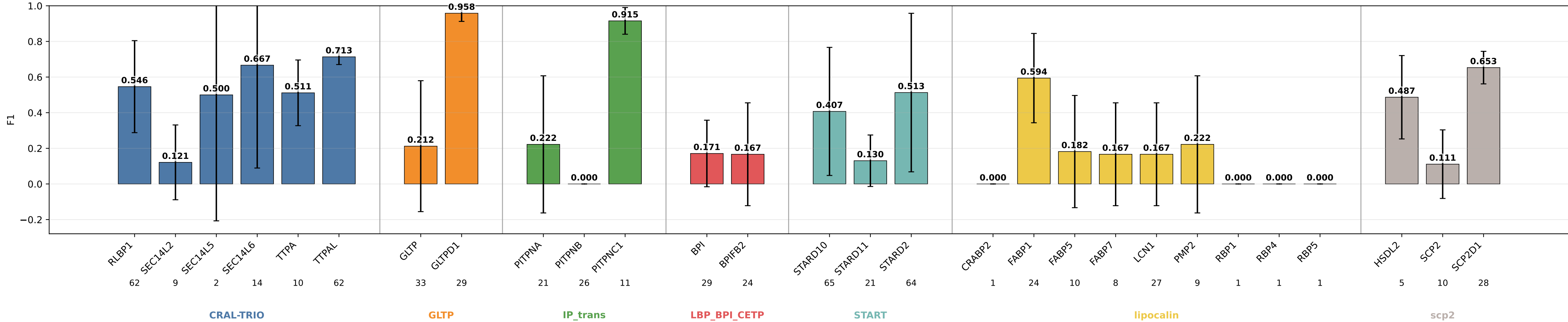
geometric_edge_mlp_protgeom8_pocket_sasa_share F1 by subgroup geometric_edge_mlp_protgeom8_pocket_sasa_share | class weights | lr=0.0001 | weight_decay=0.01 | final_m=4 | final_dropout=0.1 | hiddim=8 | heads=8 | batch=16 | ep=120 | seeds=0,1,2
