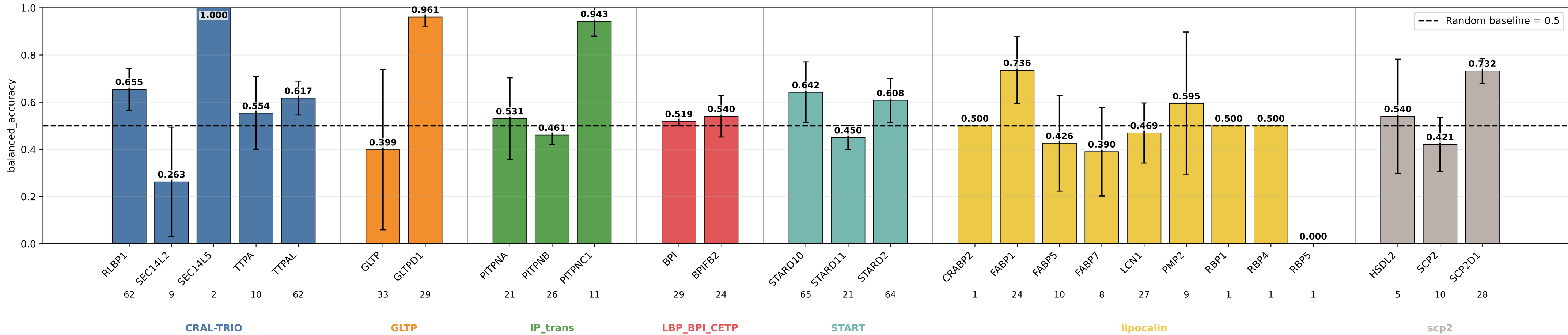
geometric_edge_mlp_protgeom8_pocket_sasa_share balanced_accuracy by subgroup geometric_edge_mlp_protgeom8_pocket_sasa_share | class weights | lr=0.0001 | weight_decay=0.01 | final_m=4 | final_dropout=0.1 | hiddim=8 | heads=8 | batch=16 | ep=120 | seeds=0,1,2
