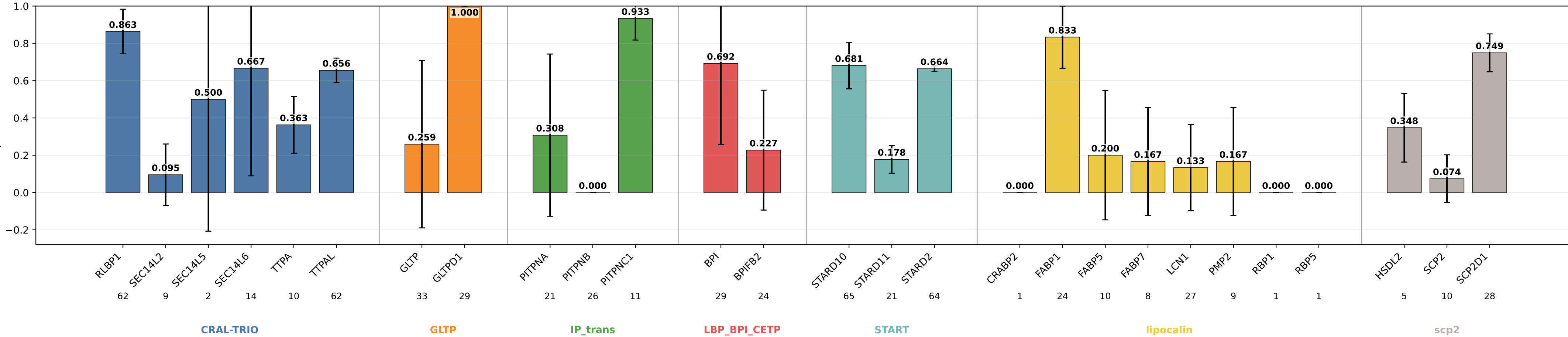
geometric_edge_mlp_protgeom8_pocket_sasa_share precision by subgroup geometric_edge_mlp_protgeom8_pocket_sasa_share | class weights | lr=0.0001 | weight_decay=0.01 | final_m=4 | final_dropout=0.1 | hiddim=8 | heads=8 | batch=16 | ep=120 | seeds=0,1,2
