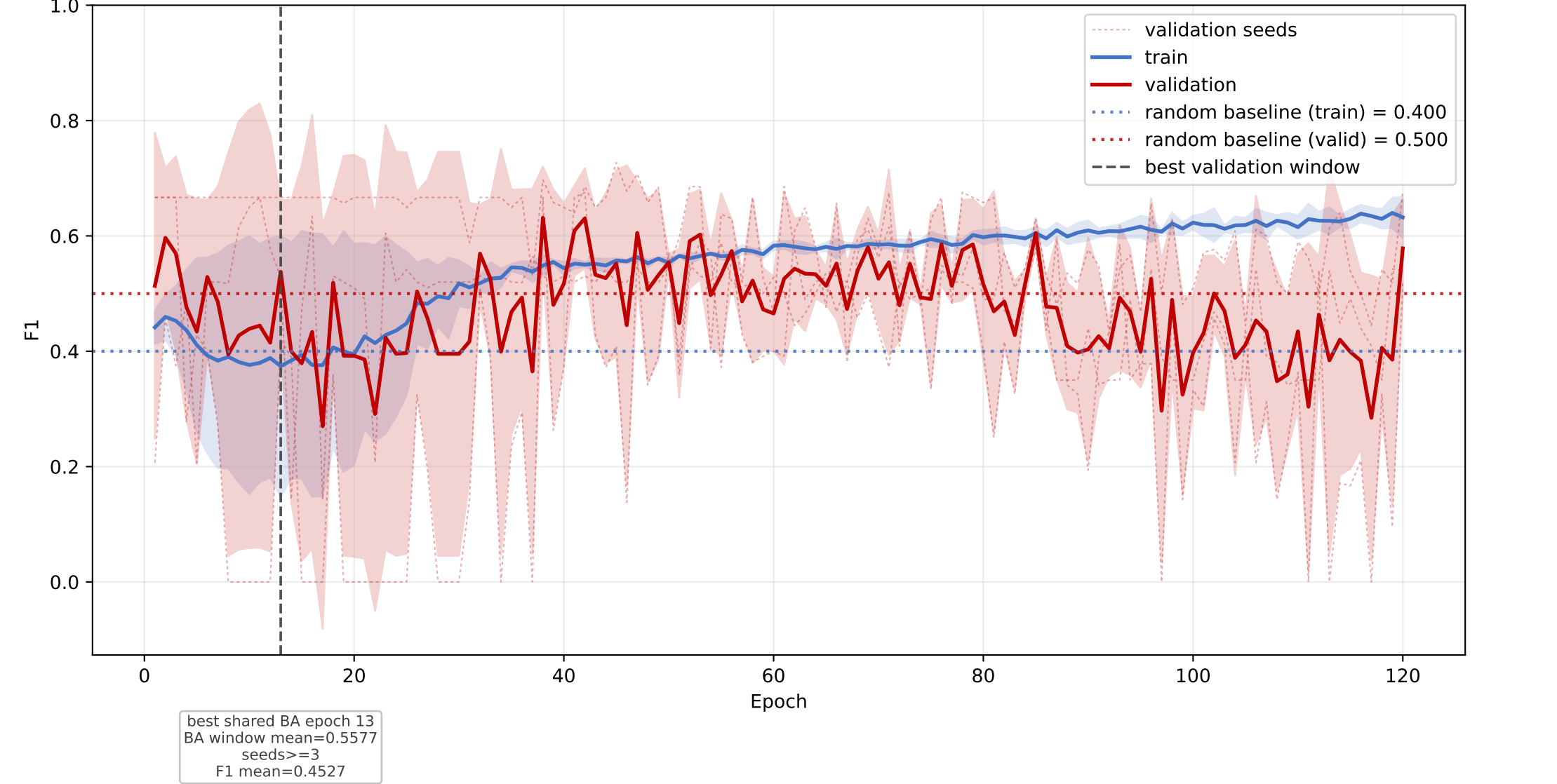
GLTP: mean F1 learning curve across seeds
