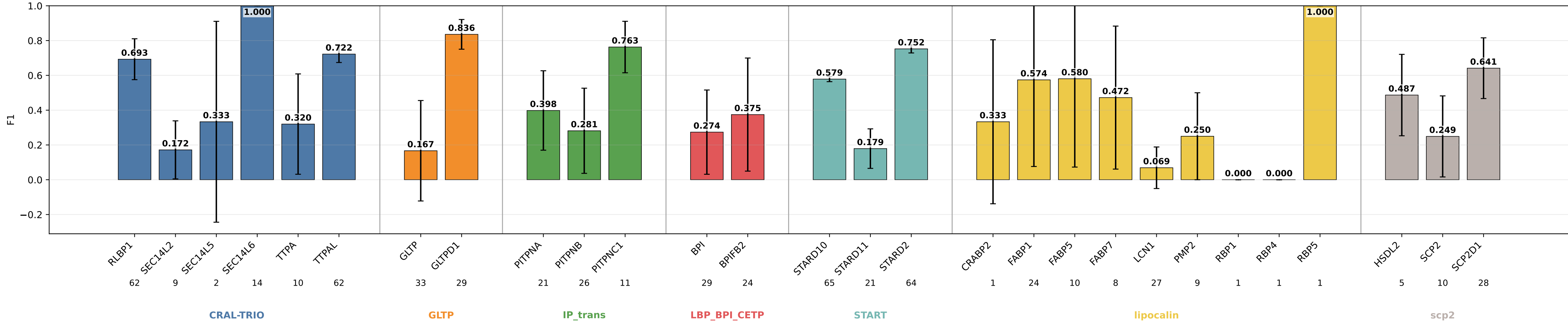
geometric_edge_mlp_protgeom8_v2 F1 by subgroup geometric_edge_mlp_protgeom8_v2 | class weights | lr=0.0001 | weight_decay=0.01 | final_m=4 | final_dropout=0.1 | hiddim=8 | heads=8 | batch=16 | ep=120 | seeds=0,1,2
