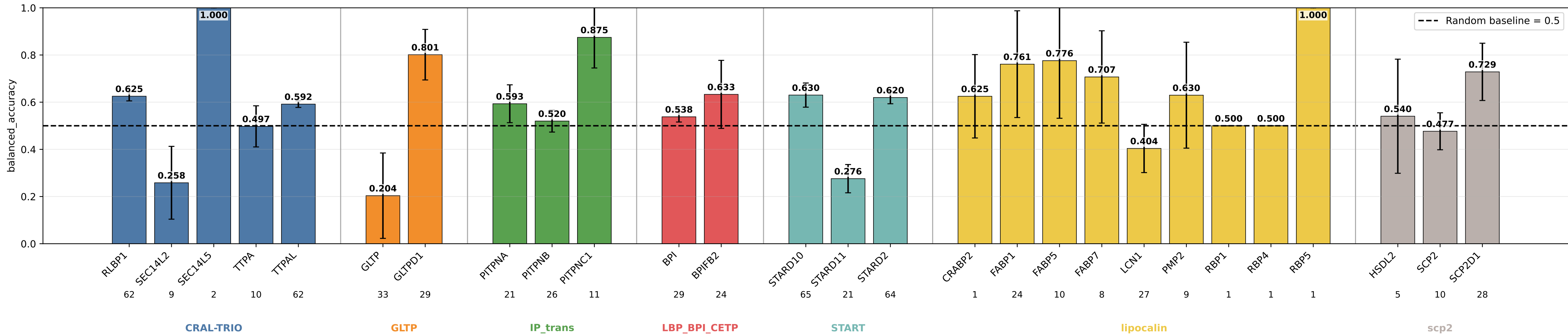
geometric_edge_mlp_protgeom8_v2 balanced_accuracy by subgroup geometric_edge_mlp_protgeom8_v2 | class weights | lr=0.0001 | weight_decay=0.01 | final_m=4 | final_dropout=0.1 | hiddim=8 | heads=8 | batch=16 | ep=120 | seeds=0,1,2
