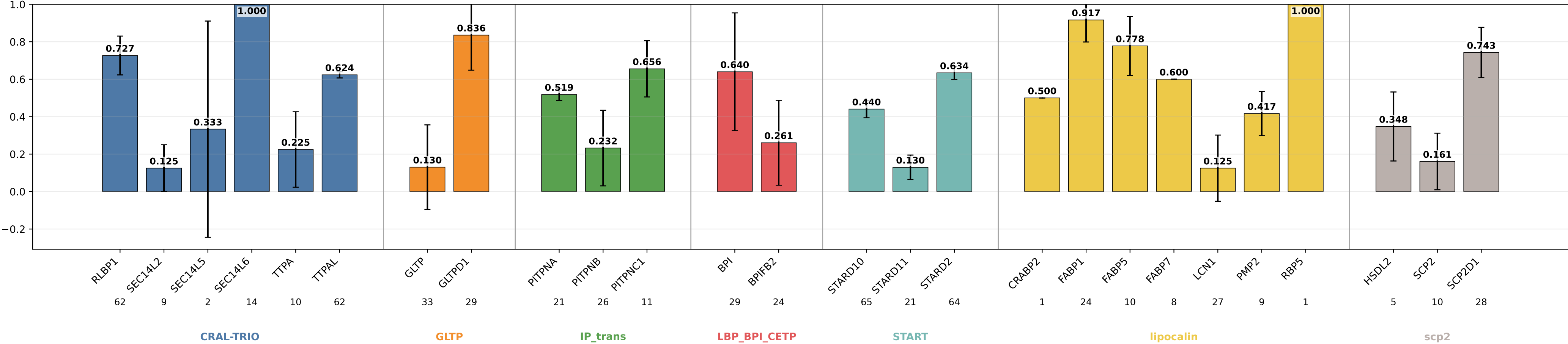
geometric_edge_mlp_protgeom8_v2 precision by subgroup geometric_edge_mlp_protgeom8_v2 | class weights | lr=0.0001 | weight_decay=0.01 | final_m=4 | final_dropout=0.1 | hiddim=8 | heads=8 | batch=16 | ep=120 | seeds=0,1,2
