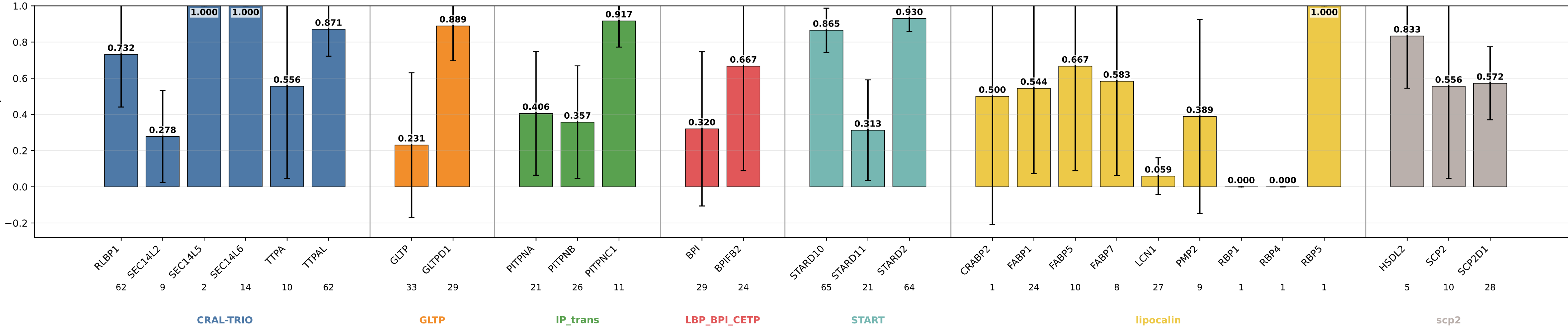
geometric_edge_mlp_protgeom8_v2 sensitivity by subgroup geometric_edge_mlp_protgeom8_v2 | class weights | lr=0.0001 | weight_decay=0.01 | final_m=4 | final_dropout=0.1 | hiddim=8 | heads=8 | batch=16 | ep=120 | seeds=0,1,2
