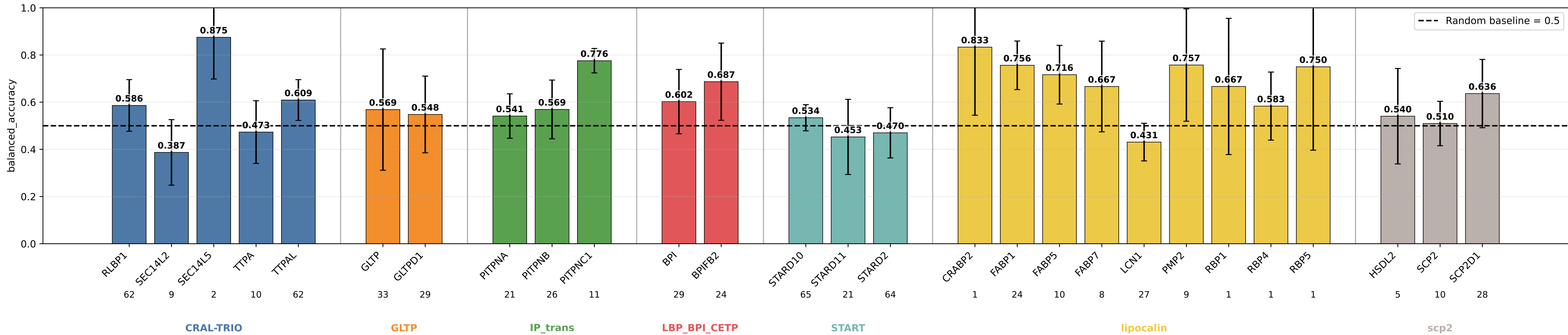
geometric_edge_mlp_protgeom_family_neutral_bilinear_fusion balanced_accuracy by subgroup geometric_edge_mlp_protgeom_family_neutral_bilinear_fusion | class weights | lr=0.0001 | weight_decay=0.01 | final_m=4 | final_dropout=0.1 | hiddim=8 | heads=8 | batch=16 | ep=120 | seeds=0,1,2,3,4
