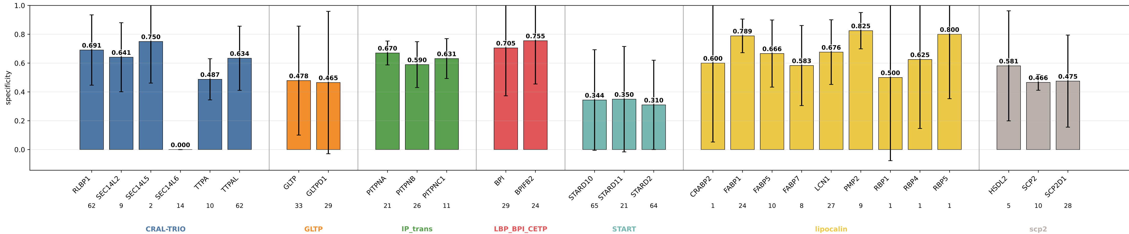
geometric_edge_mlp_protgeom_family_neutral_bilinear_fusion specificity by subgroup geometric_edge_mlp_protgeom_family_neutral_bilinear_fusion | class weights | lr=0.0001 | weight_decay=0.01 | final_m=4 | final_dropout=0.1 | hiddim=8 | heads=8 | batch=16 | ep=120 | seeds=0,1,2,3,4
