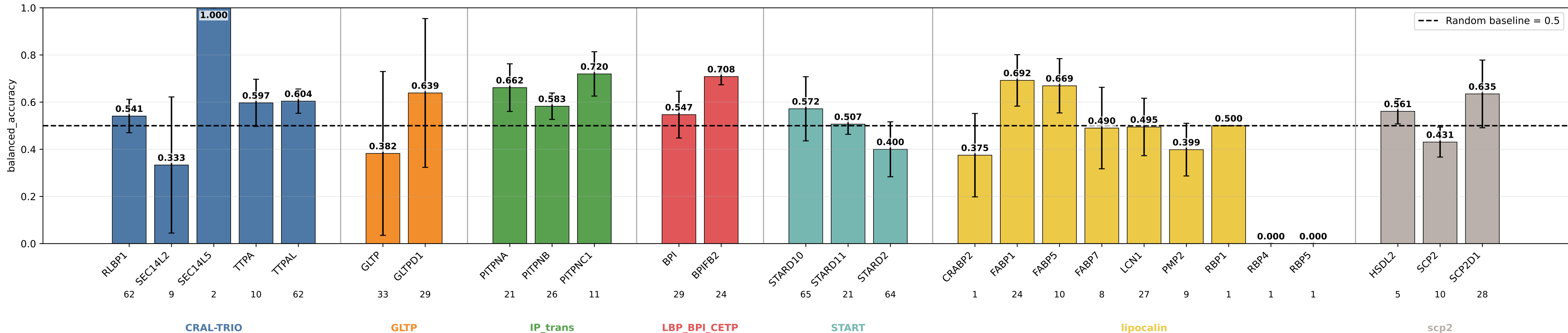
geometric_edge_mlp_protgeom_normalized_dro_wd01 balanced_accuracy by subgroup geometric_edge_mlp_protgeom_normalized_dro_wd01 | class weights | lr=0.0001 | weight_decay=0.1 | final_m=4 | final_dropout=0.1 | hiddim=8 | heads=8 | batch=16 | ep=120 | seeds=0,1,2
